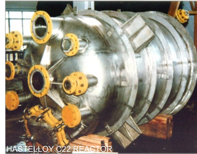
HASTELLOY C22 REACTOR
